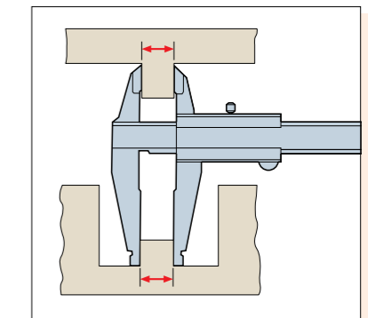
For pipe thickness measurement
