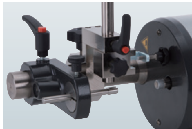
Application for mounting bore gage accessory set (type C) Order No. 02ASU162
